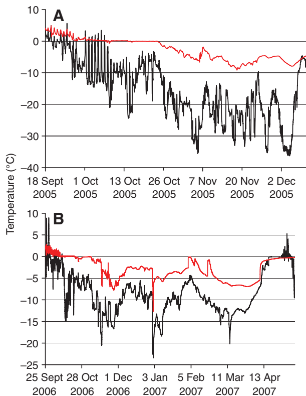
Fig. 1. Stream temperatures measured at the sediment–water interface (red) and the air or ground level temperatures (black) from the headwaters of the Chandalar River located near the Atigun Pass in the Brooks Range, AK, USA. (A) Temperature data from the winter of 2005–2006 was truncated due to a logger failure. Black tracing represents air temperature. (B) Winter 2006–2007. Black tracing indicates temperature at ground level; midwinter ground-level temperatures are higher than air temperatures due to the insulating effect of snow cover.
