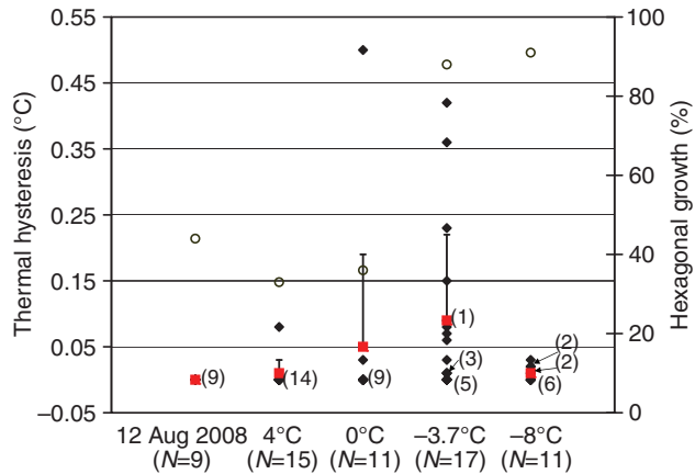
Fig. 4. Thermal hysteresis and percent hexagonal crystal growth versus acclimation or acclimatization. Insects were either field collected or acclimated to various temperatures, which are indicated along the x-axis. The insects were bled and their hemolymph was assayed for thermal hysteresis (TH) and hexagonal crystal growth morphology. Black diamonds represent individual TH measurements, and the numbers in parentheses indicate the number of overlapping data points. Red squares represent the mean TH, and error bars indicate 1 s.d. Open circles correspond to the secondary y-axis and indicate the percent of nymphs that exhibited hexagonal crystal growth morphology in their hemolymph.
