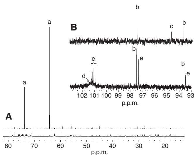
Fig. 3. Partial 13 C{ 1 H} NMR spectra (150 MHz) comparing the whole-body homogenates of warm-acclimated (4°C) and cold-acclimated (-8°C) insects. The lower spectrum in each alignment represents the homogenate from warm-acclimated nymphs ( N=30 ) and the upper spectrum represents cold-acclimated nymphs ( N=30 ). (A) Expansion of the region between 12.5 and 82 p.p.m. (B) Expansion of saccharide anomeric region. Reduced signal-to-noise ratio due to lower signal intensity. Assignment of the signals are as follows: a, glycerol; b, glucose ( \alpha and \beta anomers); c, \alpha,\alpha -trehalose; d, glycogen – broad hump in the baseline; e, tentative glucose oligomers produced from degradation of glycogen.
