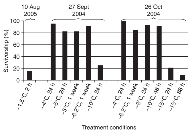
Fig. 2. Survivorship of N. arctica nymphs collected in late summer and early autumn. The collection dates are shown at the top of the figure. Nymphs were frozen in sealed plastic bags partially filled with water. The duration and temperature of the treatments (indicated on the x-axis) were varied according to survivorship of the nymphs collected on a specific date. Survivorship was assessed 24–48 h after complete thawing at 4°C.
