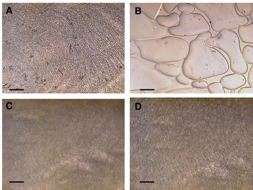
Fig. 5. Comparison of recrystallization of ice crystals in pooled hemolymph ( N=10 ) from nymphs collected in September 2007 and acclimated to -5.7^{\circ}\text{C} versus ice in a buffer control, consisting of 25\text{ mmol l}^{-1} Tris buffer, 1\text{ mg ml}^{-1} BSA and 0.5\text{ mol l}^{-1} glycerol. The melting point of the hemolymph and the control buffer were approximately equal. (A) Control buffer initial time point; (B) Control buffer after annealing; (C) N. arctica hemolymph at initial time point; (D) N. arctica hemolymph after annealing. Samples were frozen by cooling at 40^{\circ}\text{C min}^{-1} to -30^{\circ}\text{C} . The initial picture was taken after the sample froze and was warmed to -6^{\circ}\text{C} . The sample was allowed to anneal at -6^{\circ}\text{C} for 6 h before the second picture was taken. Scale bars, 100\text{ }\mu\text{m} .
