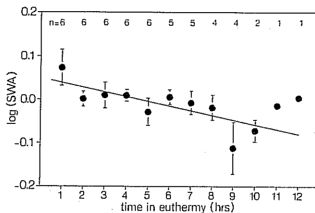
Fig. 3. Time course of slow-wave activity (SWA) during the first 12 h of 6 arousals in 3 hibernating arctic ground squirrels. Means ( \pm S.E.M.) of the values for different arousals are shown.
